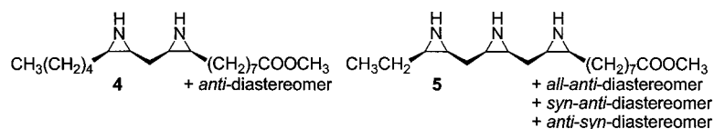
Figure 1. Bis(aziridine) 4 , based on methyl linoleate, and tris(aziridine) 5 , based on methyl linolate [1]
