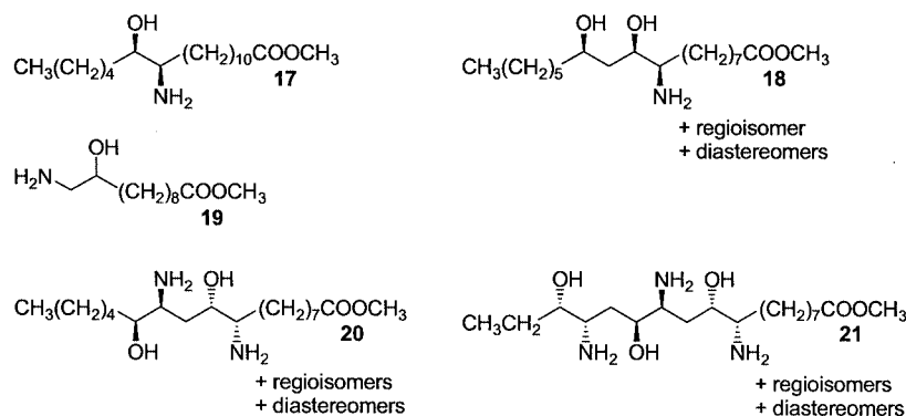
Figure 3. New fatty amino alcohols 17–21 prepared by reduction of the corresponding azido alcohols
