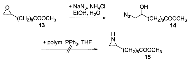
Scheme 6. Conversion of methyl 10,11-epoxyundecanoate ( 13 ) into methyl 11-azido-10-hydroxyundecanoate ( 14 ) and the failed transformation to the terminal aziridine 15
