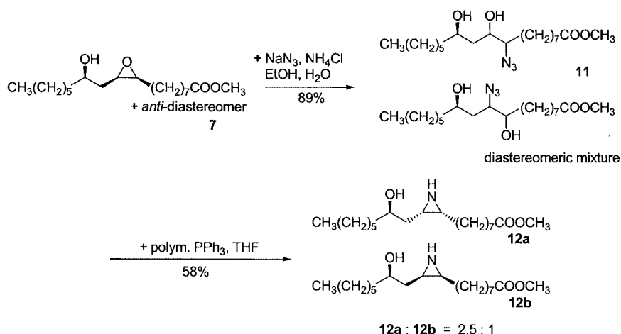
Scheme 5. Synthesis of methyl (9 R ,10 S ,12 R )-9,10-epimino-12-hydroxyoctadecanoate ( 12a ) and methyl (9 S ,10 R ,12 R )-9,10-epimino-12-hydroxyoctadecanoate ( 12b ) from methyl epoxyricinoleate ( 7 ) via the regio- and diastereomeric azido diols 11
