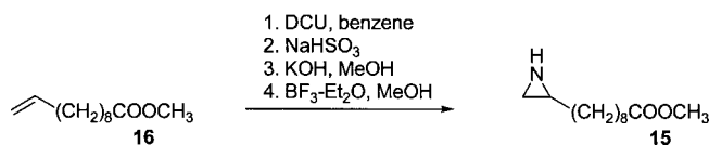
Scheme 7. Synthesis of methyl 10,11-epiminoundecanoate ( 15 ) by the DCU method, starting from methyl 10-undecenoate ( 16 )
