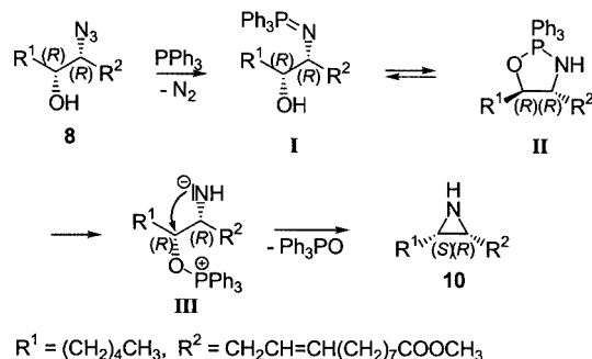
Scheme 4. Stereochemical course of the formation of the enantiomerically pure aziridine 10 starting from the ( R,R )-configured azido alcohol 8
