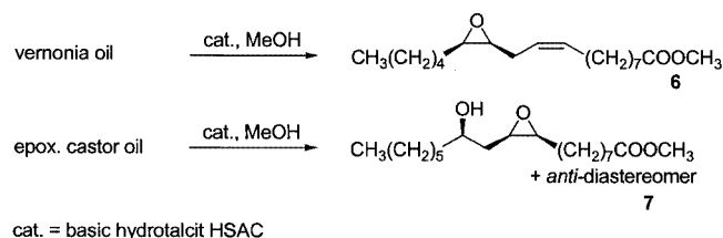
Scheme 2. Synthesis of methyl vernolate ( 6 ) and epoxidised methyl ricinoleate ( 7 ) by HSAC-catalysed transesterification of vernonia and castor oil, respectively
