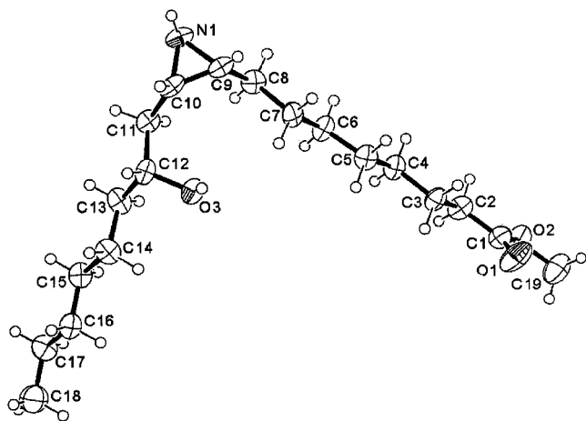
Figure 2. X-ray diffraction structure of the major diastereomer methyl (9 R ,10 S ,12 R )-9,10-epimino-12-hydroxyoctadecanoate ( 12a )
