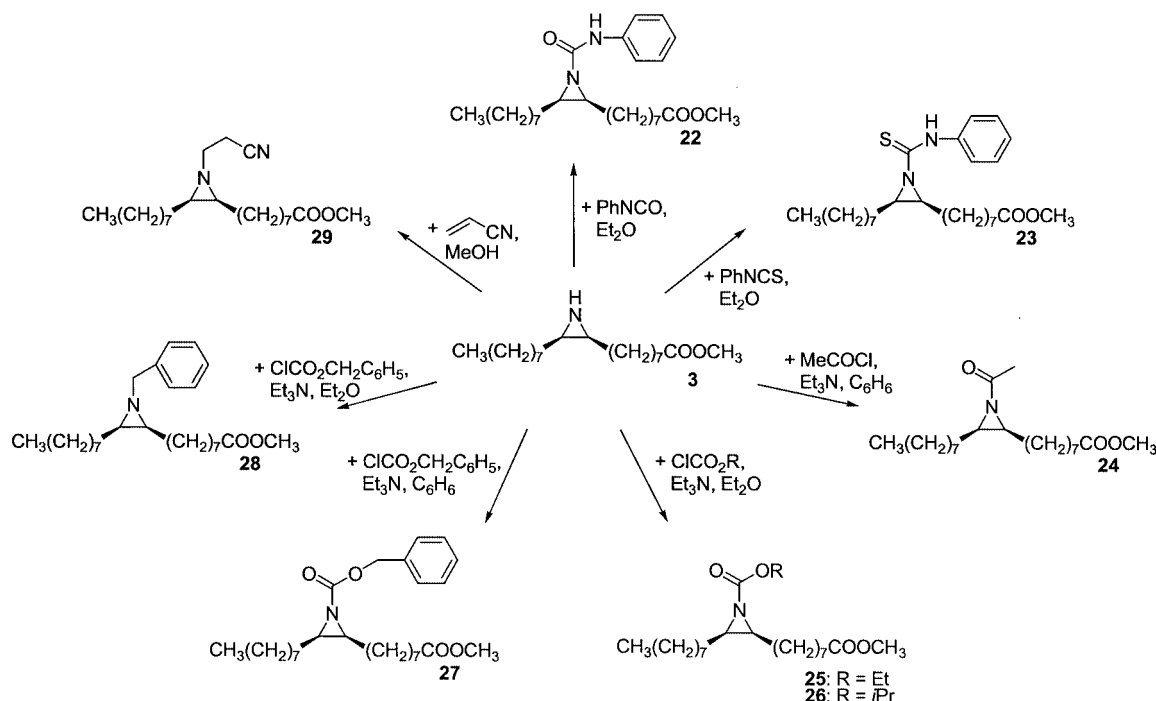
Scheme 8. Synthesis of N -substituted aziridine derivatives 22–29 from methyl cis -9,10-epiminooctadecanoate (3); for purposes of clarity the racemic compounds 3 and 22–29 are each shown as only one enantiomer
