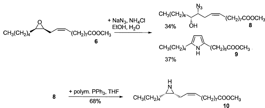
Scheme 3. Synthesis of enantiomerically pure methyl (9 Z ,12 R ,13 S )-12,13-epimino-9-octadecenoate ( 10 ), starting from methyl vernolate ( 6 ), via methyl (9 Z ,12 R ,13 R )-12-azido-13-hydroxy-9-octadecenoate ( 8 ); pyrrole 9 was obtained in equal amounts and separated by column chromatography
