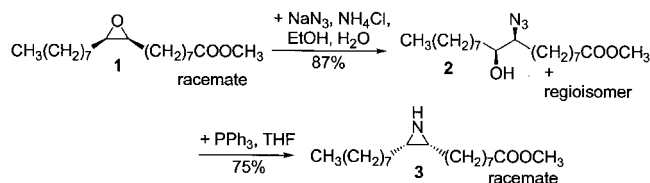
Scheme 1. Synthesis of methyl cis -9,10-epiminooctadecanoate ( 3 ), starting from methyl cis -9,10-epoxyoctadecanoate ( 1 ), via azido alcohol 2 [4]
